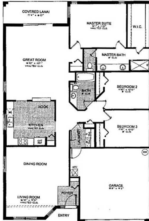
Villa Floor plan
